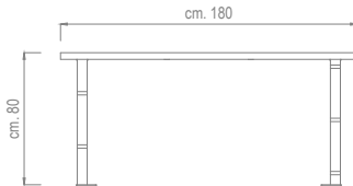
VISTA FRONTALE / FRONTAL VIEW
