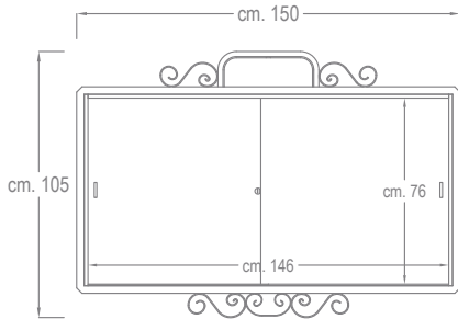
VISTA FRONTALE / FRONTAL VIEW
