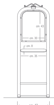
VISTA FRONTALE / FRONTAL VIEW
