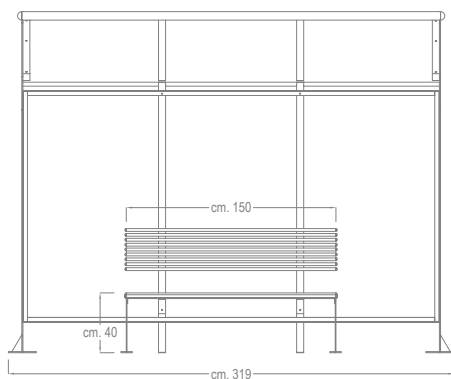
VISTA FRONTALE / FRONTAL VIEW
