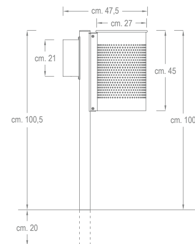
VISTA LATERALE / LATERAL VIEW
