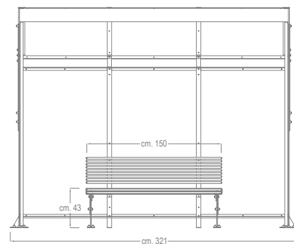
VISTA FRONTALE / FRONTAL VIEW
