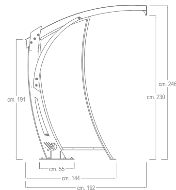
VISTA LATERALE / LATERAL VIEW
