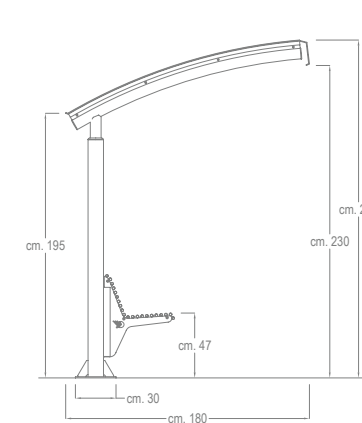
VISTA LATERALE / LATERAL VIEW
