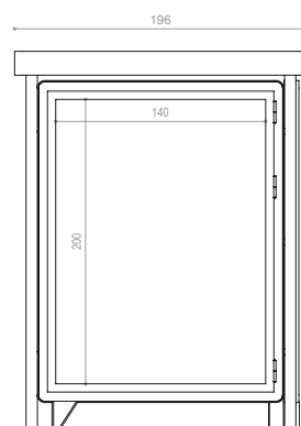
VISTA LATERALE / LATERAL VIEW
