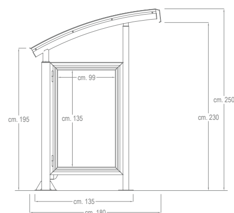
VISTA LATERALE / LATERAL VIEW
