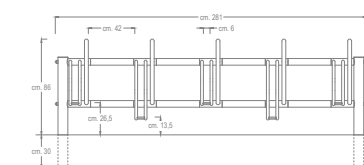
VISTA FRONTALE / FRONTAL VIEW
