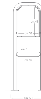
VISTA FRONTALE / FRONTAL VIEW
