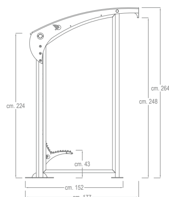
VISTA LATERALE / LATERAL VIEW
