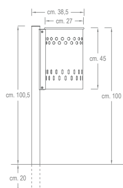
VISTA LATERALE / LATERAL VIEW
