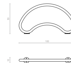
VISTA FRONTALE / FRONTAL VIEW
