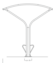
VISTA LATERALE / SIDE VIEW
